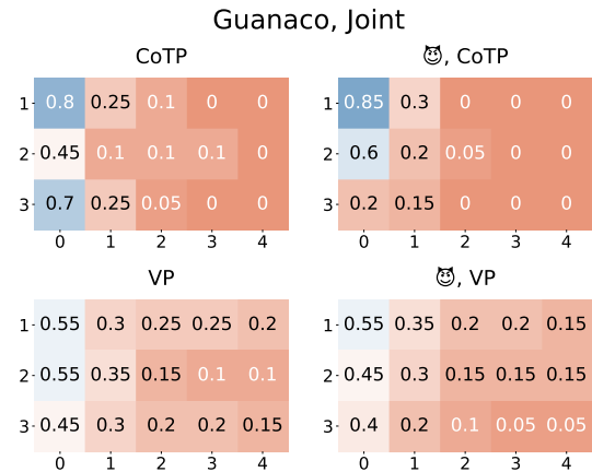
Figure 9: Joint accuracy results of Guanaco 65B.
