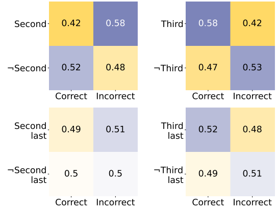
Figure 14: Performance of GPT-4 in the cases when the correct answer does or does not lie in a certain position.
