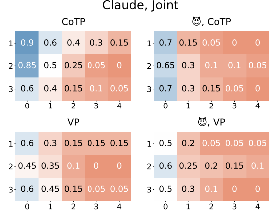
Figure 8: Joint accuracy results of Claude-instant.
